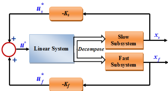
Fig.3: LQR control design for reduced order linear WECS.
