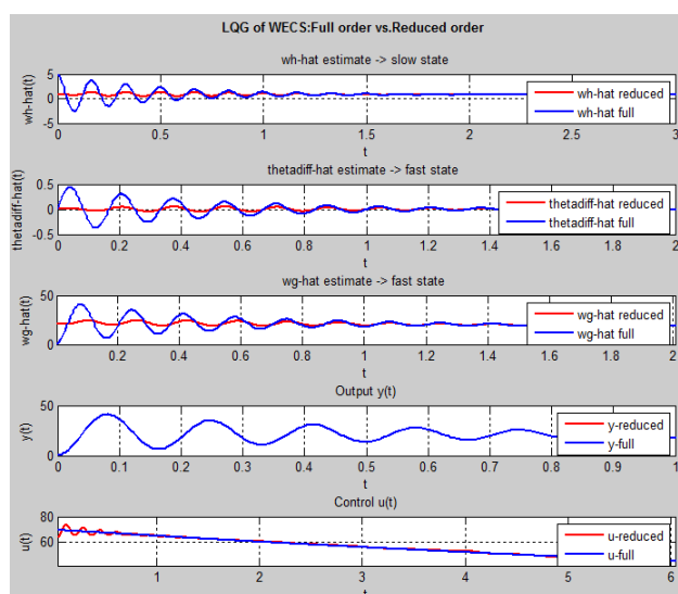
Fig.11: Detailed view of LQG comparison plots.
