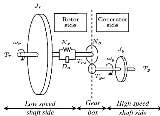
Fig.2: Schematic of the WECS [14].
