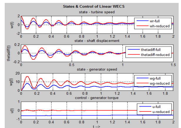
Fig.7: Detailed view of the LQR comparison plots near the origin.
