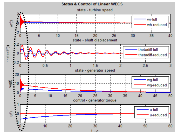
Fig.6: LQR control – Comparison of the full order system and reduced order WECS.
