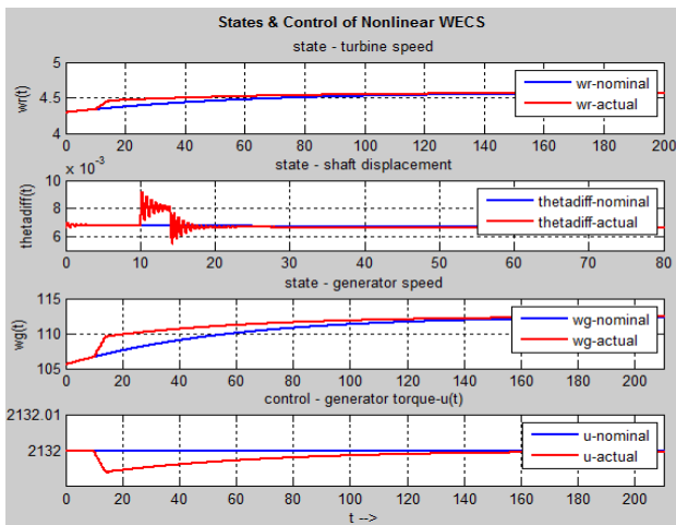
Fig.8: States and control of nonlinear WECS with composite LQR control.
