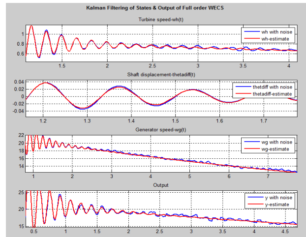
Fig.9: States and output compared to their Kalman estimates.
