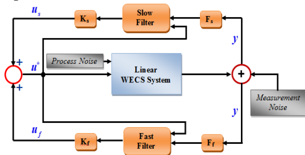
Fig.5: LQG control design of WECS with reduced order filter and regulator.
