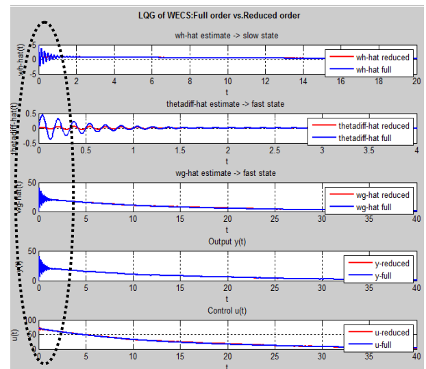
Fig.10: Comparison of full order and reduced order LQG control.
